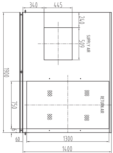
SUPPLY & RETURN VIEW
