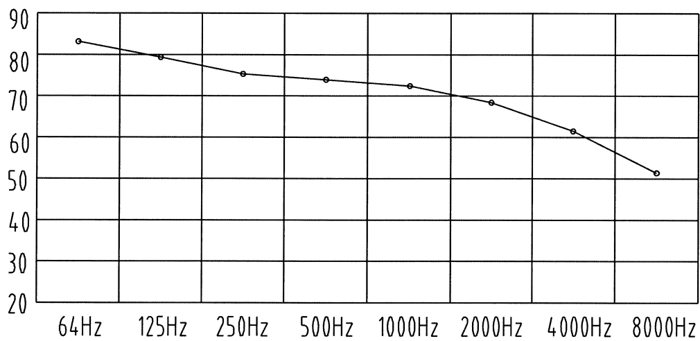
Noise rate analysing chart ( A Class: 77.2dB) dB
