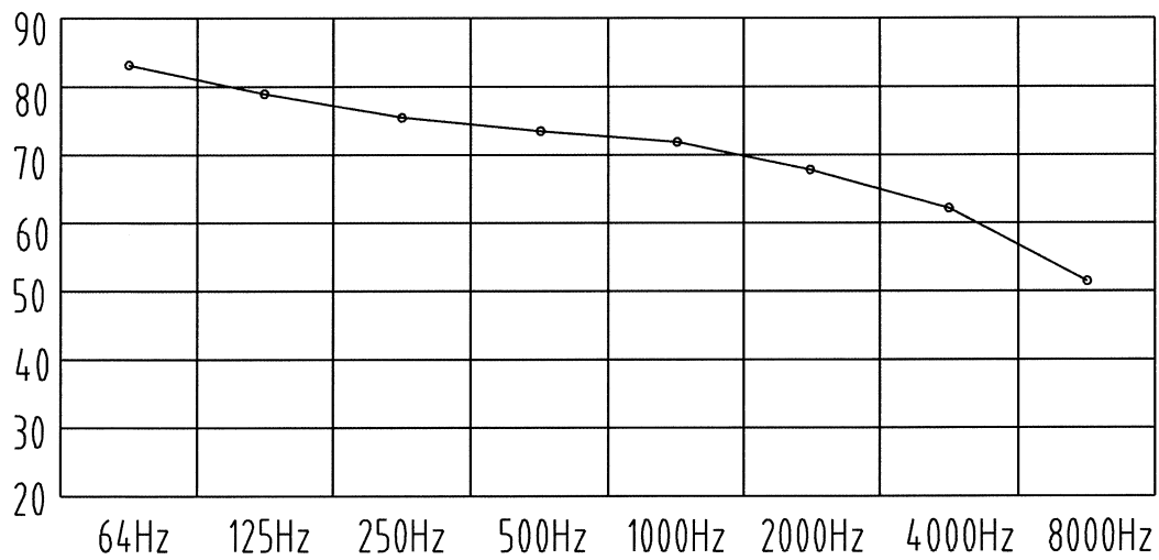
Noise rate analysing chart ( A Class: 76.3dB) dB
